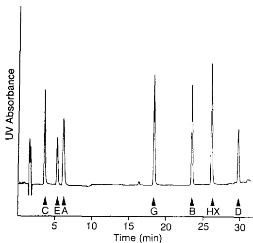
Fig. 2. Gradient HPLC separation of hexazinone and its metabolites with programmed variable-wavelength ultraviolet absorbance detection (chromatographic conditions given in text).
